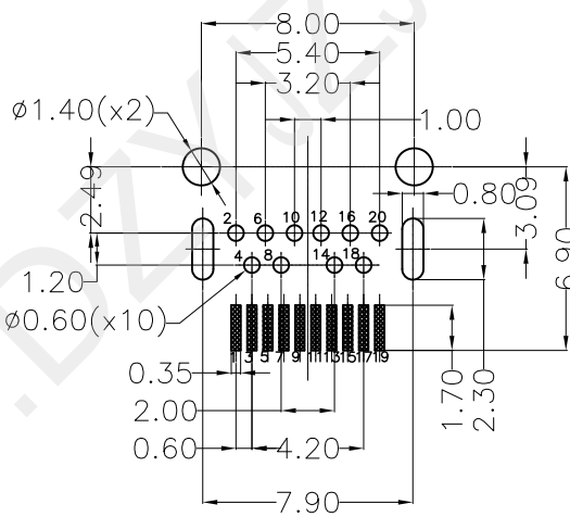
P.C.B LAYOUT (T=1.60mm) VIEW BOTTOM(tolerance±0.05)
